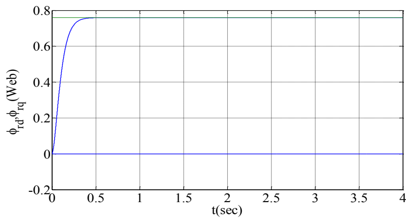
FIG. 4.9 – Flux rotoriques \phi_{rd} , \phi_{rq} .
