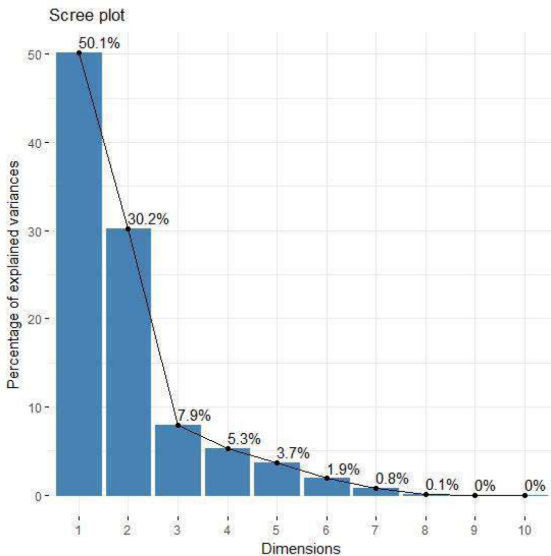
Figure 3.3 : Scree plot
