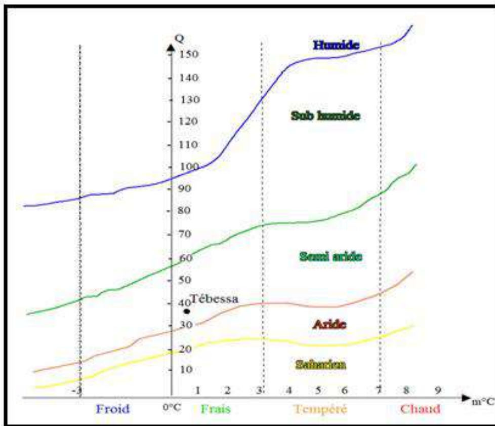
Figure 2.3: Climagramme d'EMBERGER
