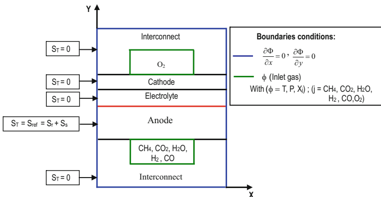
Fig. 41.1 Physical model, heat sources, and boundary conditions
