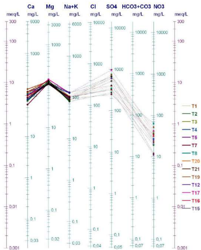
Figure 57 : Shoeller-Berkalof, Tébessa (jan 2009)
