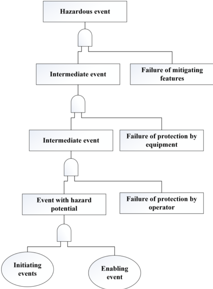
Figure 1.5: Fault tree accident model (Khan & Abbasi 1999).
